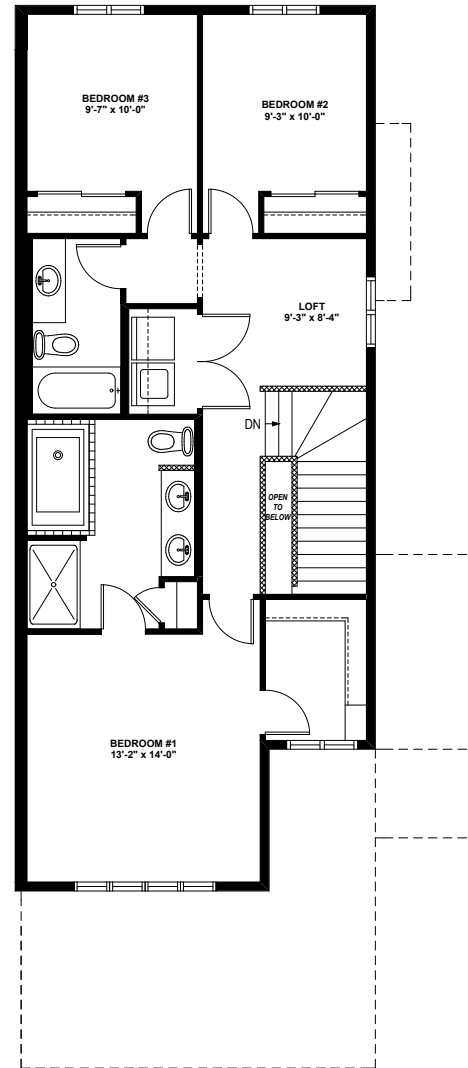
SECOND FLOOR PLAN - 887 sq.ft.
