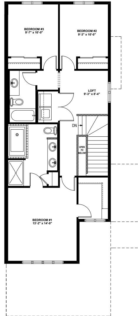
SECOND FLOOR PLAN - 881 sq.ft.
