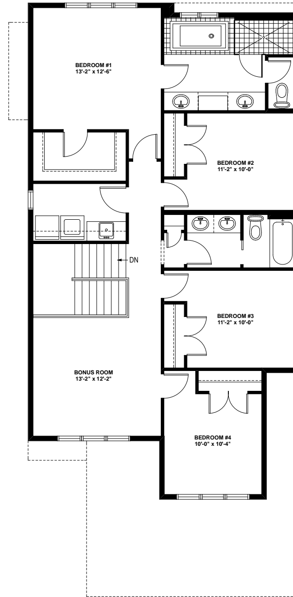
SECOND FLOOR - 1214 sq.ft.
